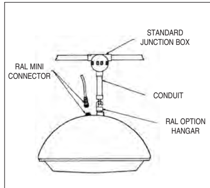
Hanger Mount with Quick Disconnect
