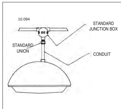
Rigid Pendant Mount with Short Conduit Hard Wired
