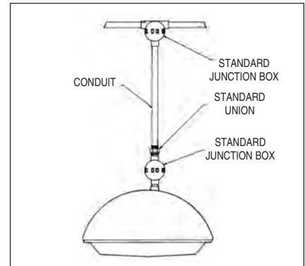
Rigid Pendant Mount with Long Conduit Hard Wired
