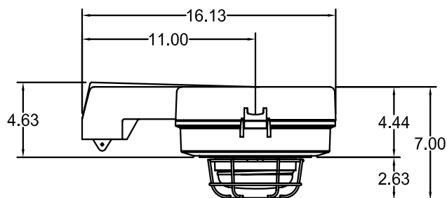
90° Stanchion mount with threaded glass globe and guard.
