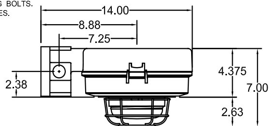
Wall mount with threaded glass globe and guard.
