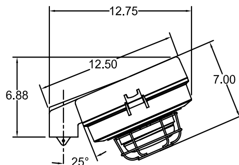
25° Stanchion mount with threaded glass globe and guard.
